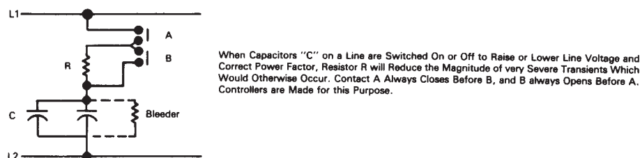
Figure 46. Power factor capacitor switching: This is usually done by public utilities to control line voltage. Switching operations create severe line transients if preinsertion resistors are not used by the utility when capacitor banks are turned on.
