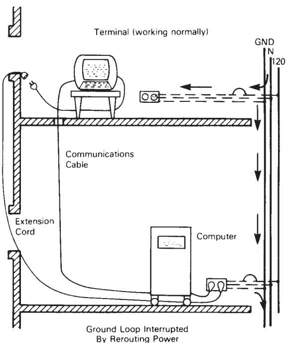
Figure 26. A temporary solution: An extension cord provides total system power from one duplex receptacle and avoids creation of a ground loop.
